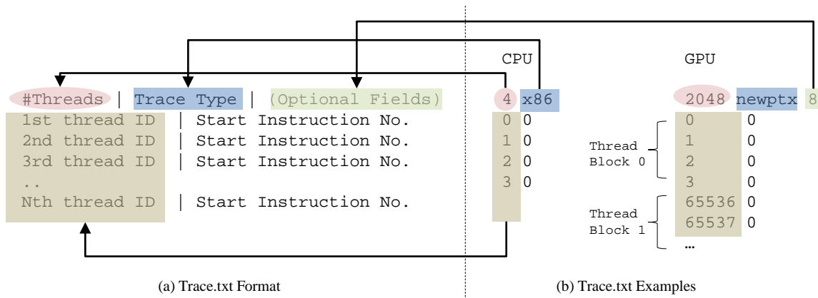
Figure 2. Trace.txt format.
