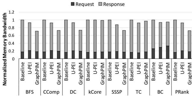
Fig. 12: Normalized bandwidth consumption with request/response breakdown
