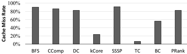
Fig. 10: Cache miss rate of offloading candidates
