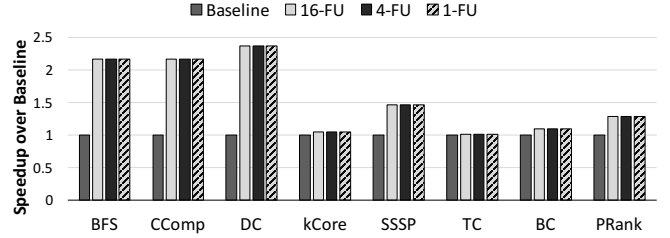
Fig. 11: Speedup over baseline system with different functional units (FU) per HMC vault
