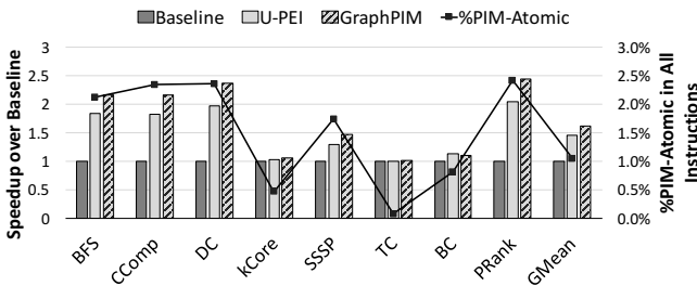
Fig. 7: Speedups over the baseline system
