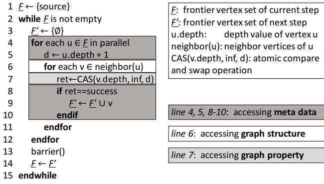
Fig. 3: Code snippet for breadth-first search (BFS)
