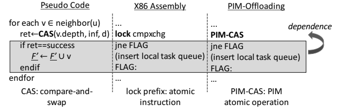
Fig. 8: Illustration of atomic instruction overhead
