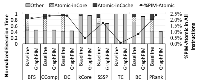
Fig. 9: Breakdown of normalized execution time (Atomic-inCore: atomic instruction cycles for pipeline freezing and write-buffer draining; Atomic-inCache: atomic instruction cycles for cache checking and coherence traffic; Other: cycles of other instructions' execution and stall)
