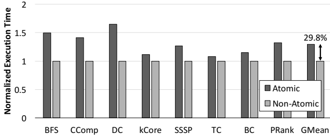
Fig. 4: Atomic instruction overhead of graph workloads on an Intel Xeon E5 machine
